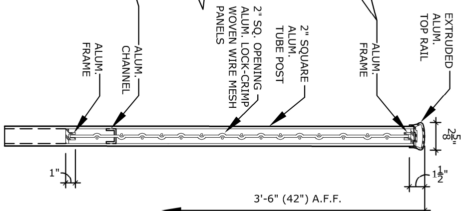
TYPICAL SECTION
