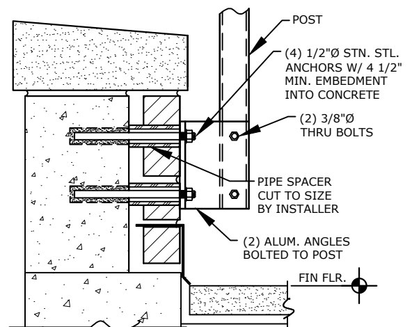
SIDE MOUNTING THROUGH BRICK VENEER (WITH ALUM. BOLTED ANGLES)
