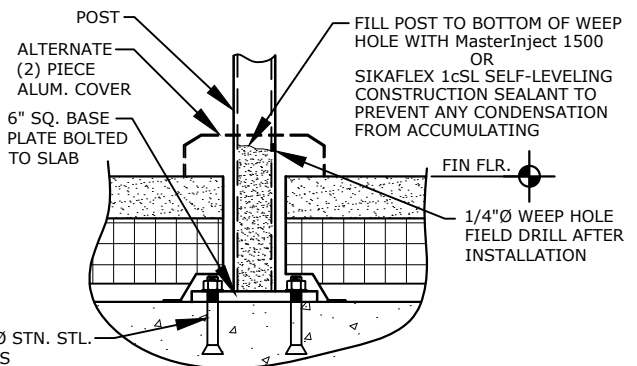
BOLT DOWN PLATE MOUNTING
