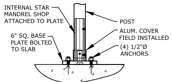
BOLT DOWN MANDREL MOUNTING
