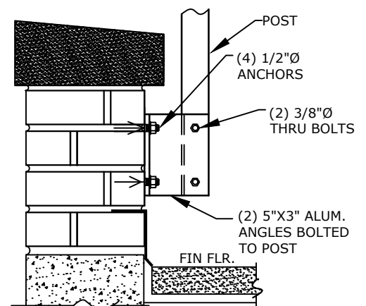
SIDE MOUNTING (WITH ALUM. BOLTED ANGLES)
