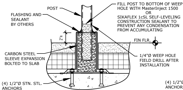
BOLT DOWN SLEEVE MOUNTING
