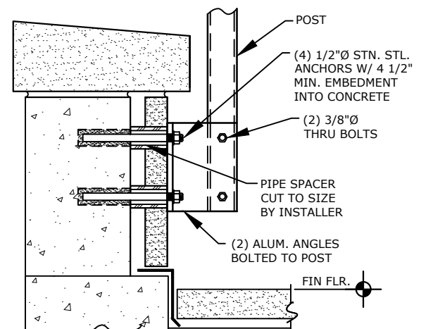
SIDE MOUNTING THROUGH STONE VENEER (WITH ALUM. BOLTED ANGLES)
