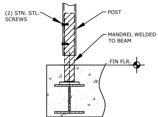
WELDED MANDREL MOUNTING
