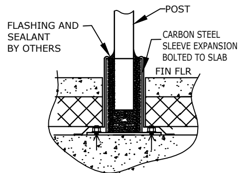
BOLT DOWN SLEEVE MOUNTING
