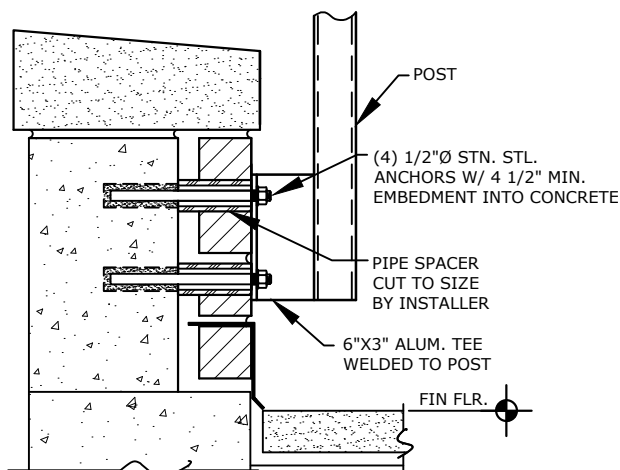
SIDE MOUNTING THROUGH BRICK VENEER (WITH ALUM. WELDED TEE)
