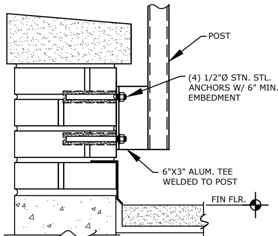
SIDE MOUNTING TO BRICK (WITH ALUM. WELDED TEE)
