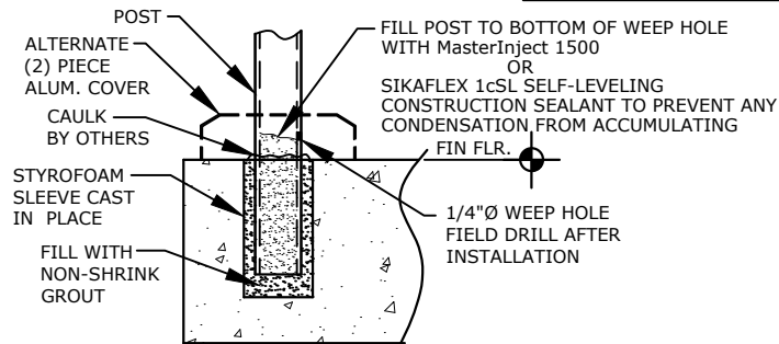
CAST IN SLEEVE MOUNTING IN CONCRETE
