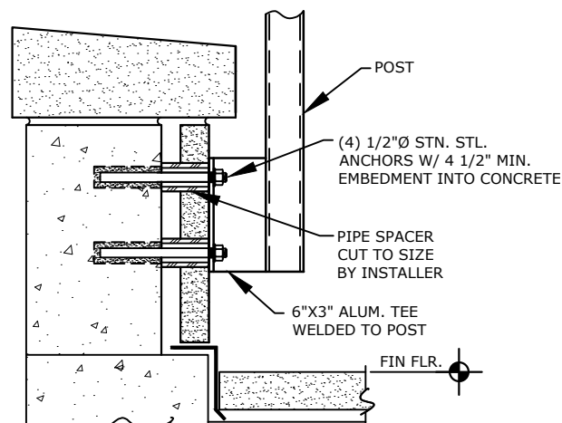
SIDE MOUNTING THROUGH STONE VENEER (WITH ALUM. WELDED TEE)
