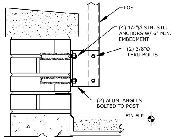
SIDE MOUNTING TO BRICK (WITH ALUM. BOLTED ANGLES)
