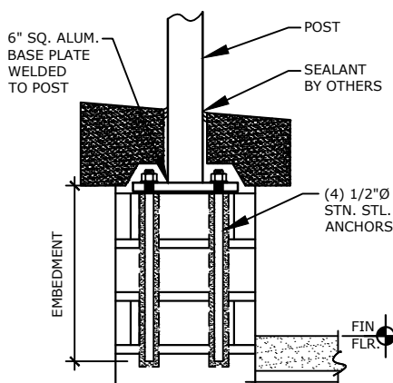
TOP MOUNTING THROUGH COPING
