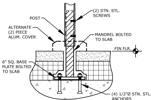
BOLT DOWN MANDREL MOUNTING
