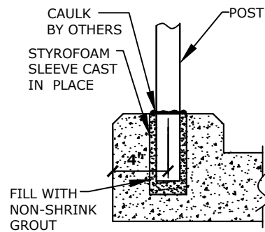
CAST IN SLEEVE MOUNTING IN CONCRETE CURB
