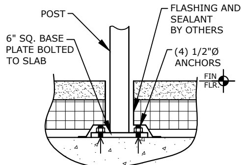
BOLT DOWN PLATE MOUNTING
