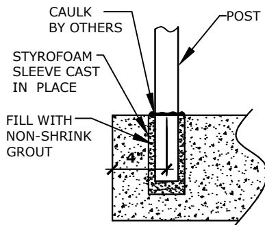
CAST IN SLEEVE MOUNTING IN CONCRETE
