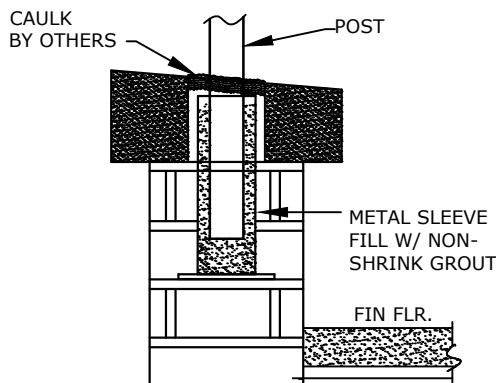
BUILT-IN SLEEVE MOUNTING IN MASONRY
