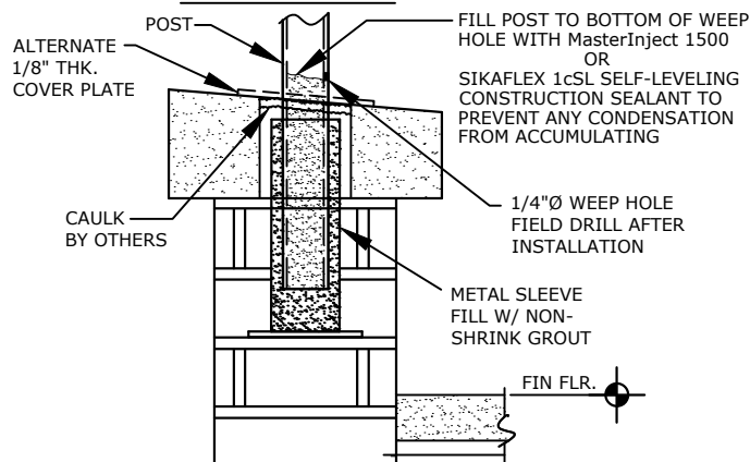
BUILT-IN SLEEVE MOUNTING IN MASONRY
